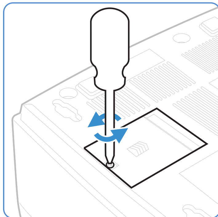
Loosen screw and open door
