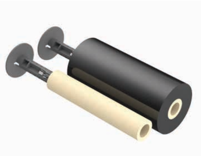
Ribbon Adapter for Notchless Ribbon Cores 205-188-010 12.7 mm (0.5 in) Ribbon Core Adapters
