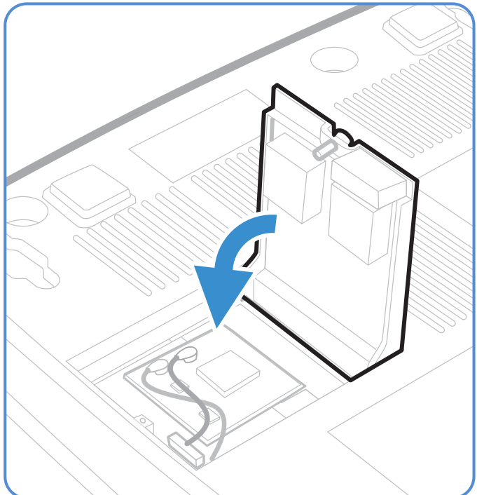
PC42E-T - Adhere antenna
