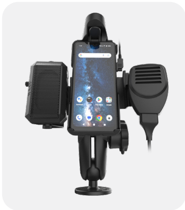
RAM-138-S-SNM5PL-V7B1U Sonim XP Pro with Speaker and Hardware
